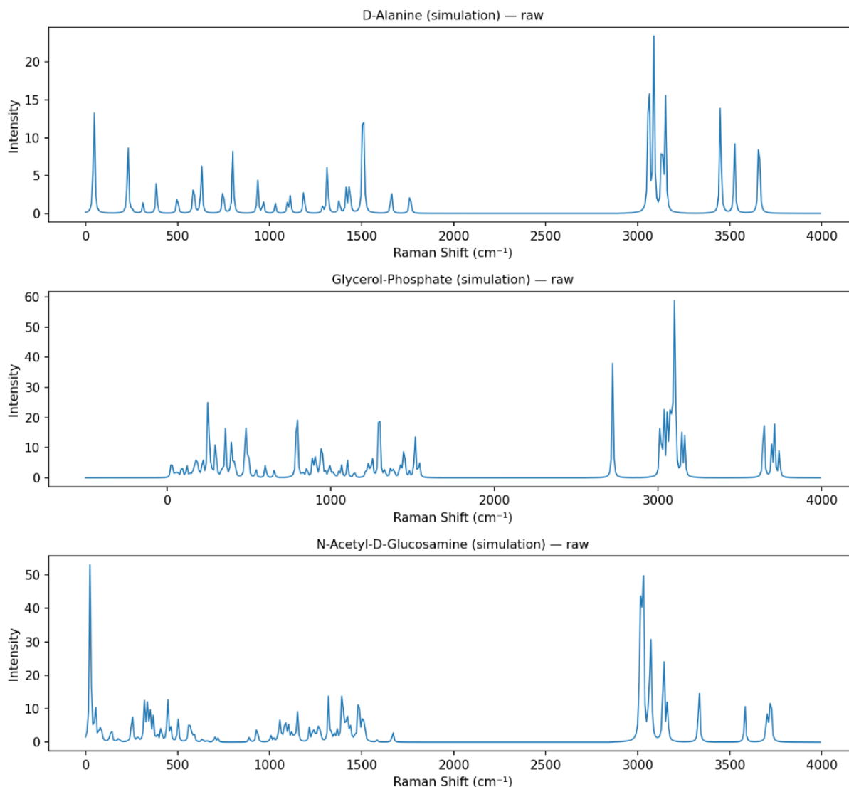
Figure 4.11: Simulated Raman spectra of individual LTA fragments: Glycerol-Phosphate, D-Alanine, and GlcNAc.
